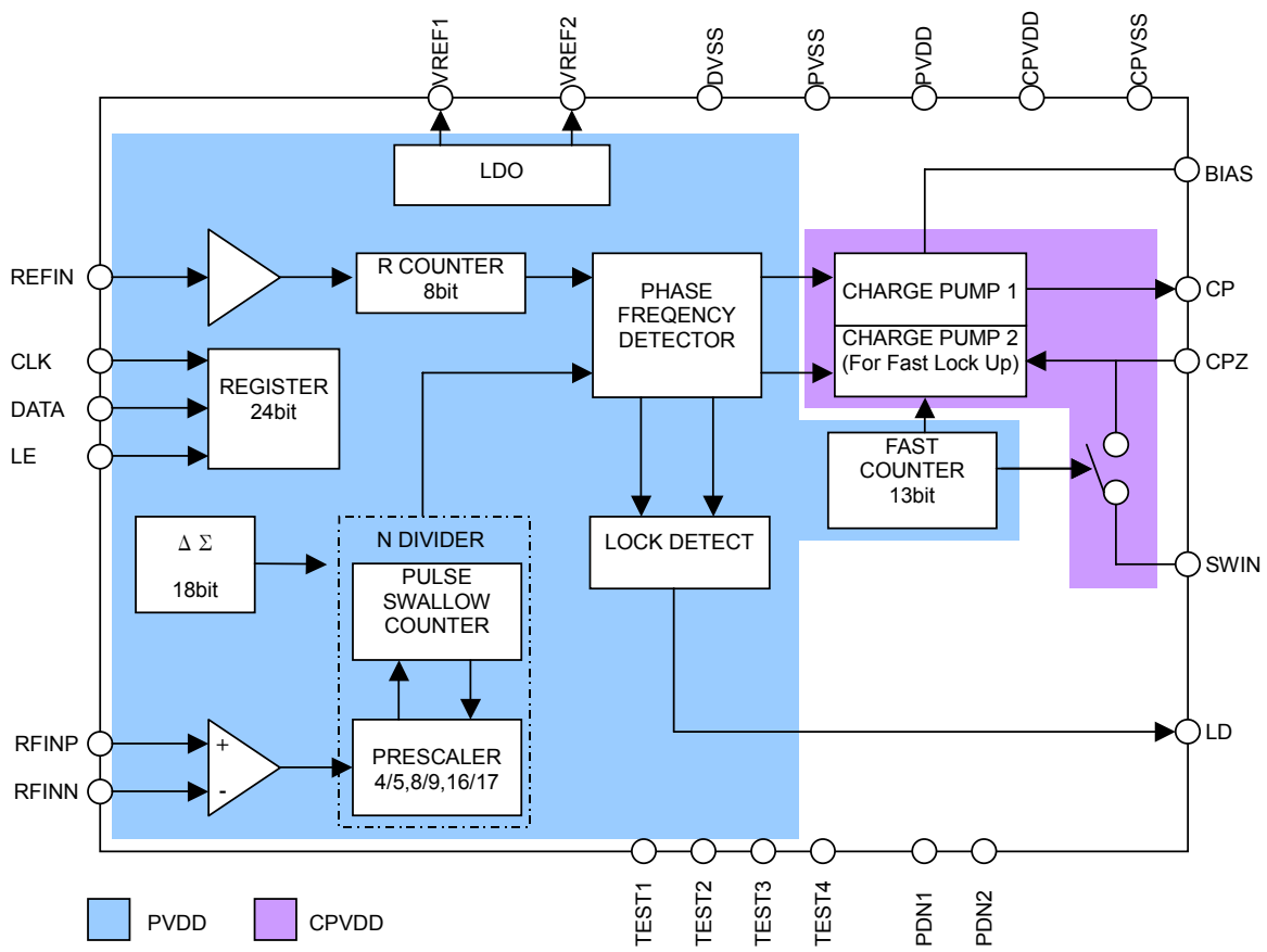
Fig. 14 Block Diagram by Power Supply
