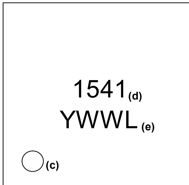
Fig. 16 Marking
