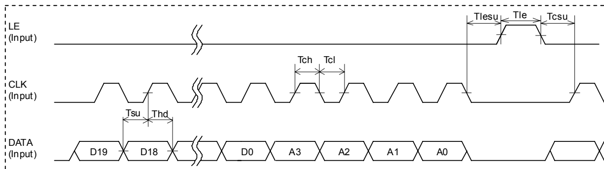
Fig. 3 Serial Interface Timing
