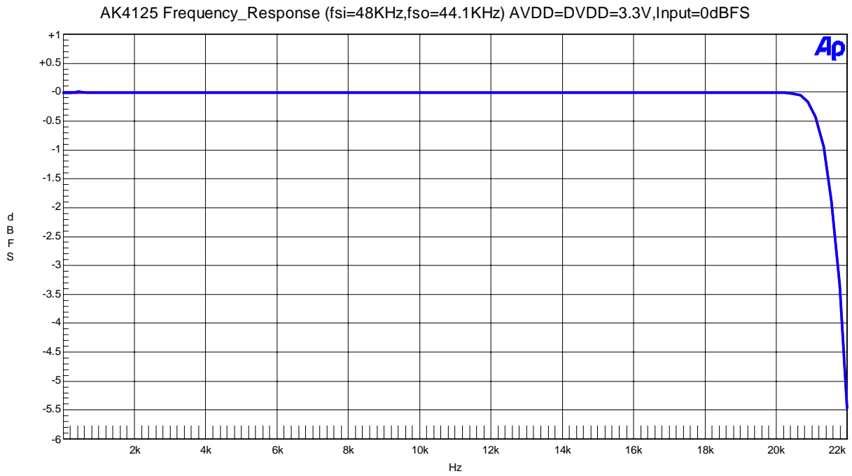
Fig 5. Frequency Response
