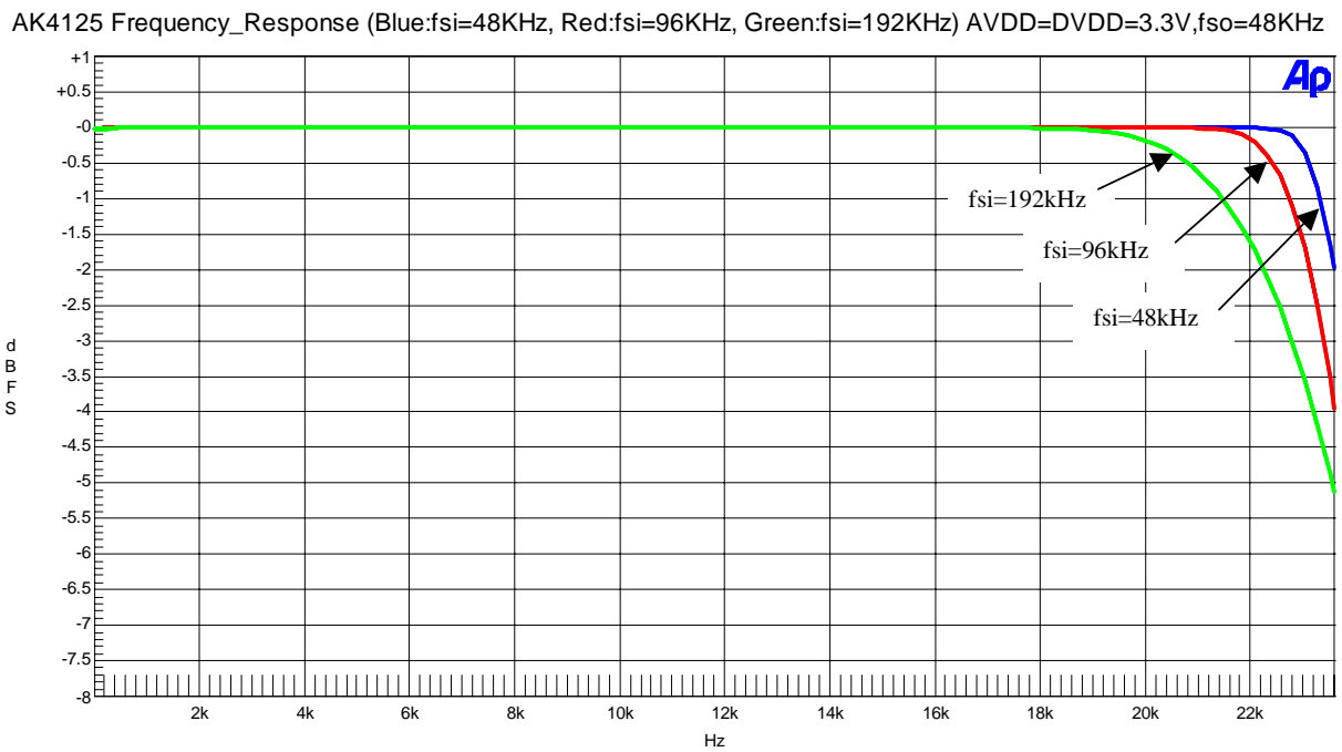
Fig 8. Frequency Response
