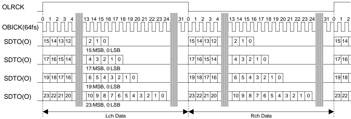
Figure 8. MSB Timing
