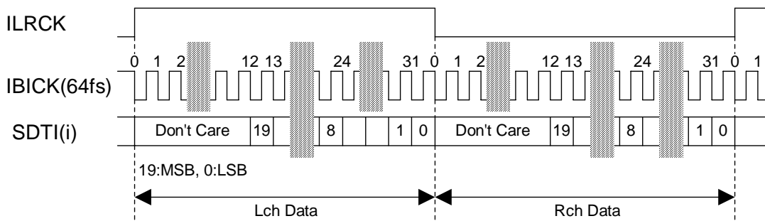
Figure 3. Mode 1 Timing
