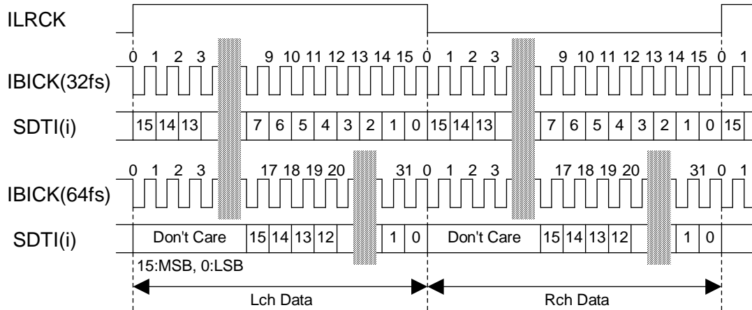
Figure 2. Mode 0 Timing
