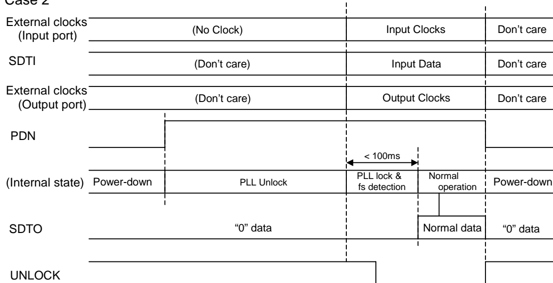
Figure 13. System Reset 2
