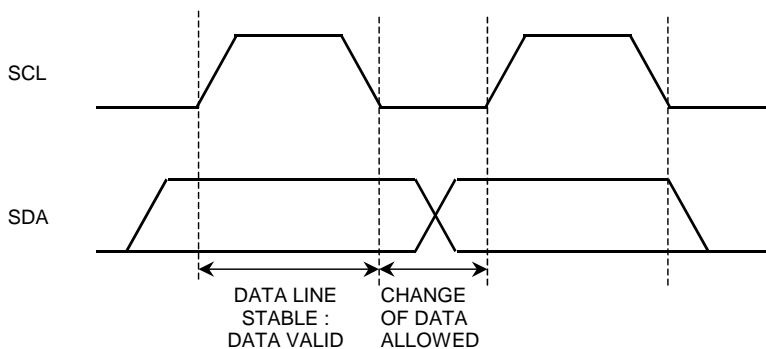
Figure 16. Data transfer
