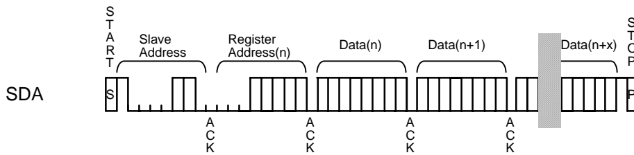
Figure 22. WRITE Operation
