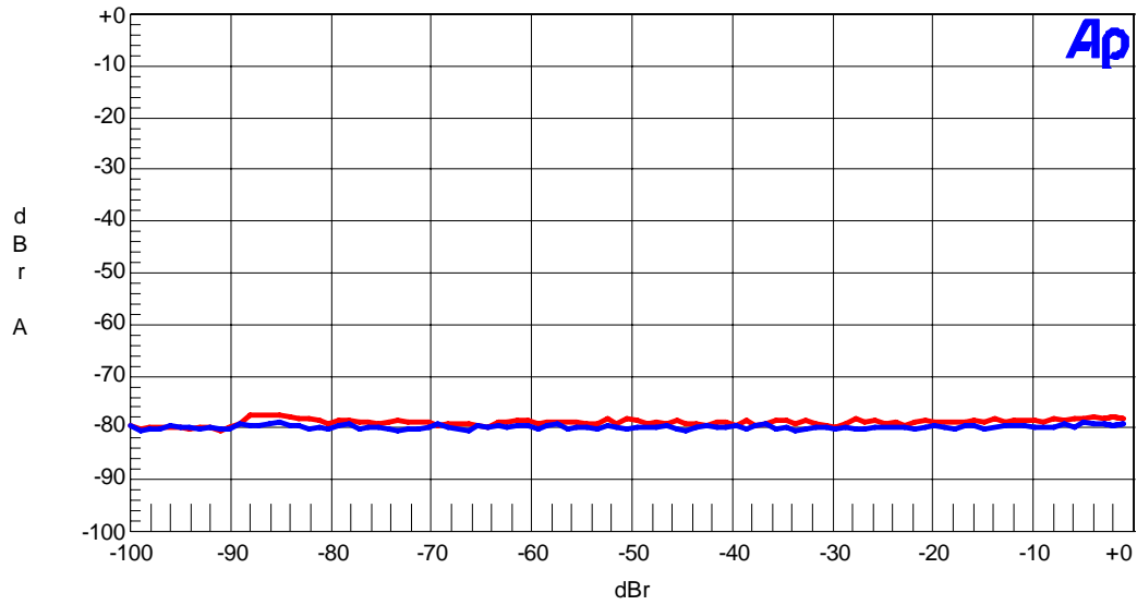
Figure. 9 Stereo mode THD + N vs. Input Level (fin=1kHz)
