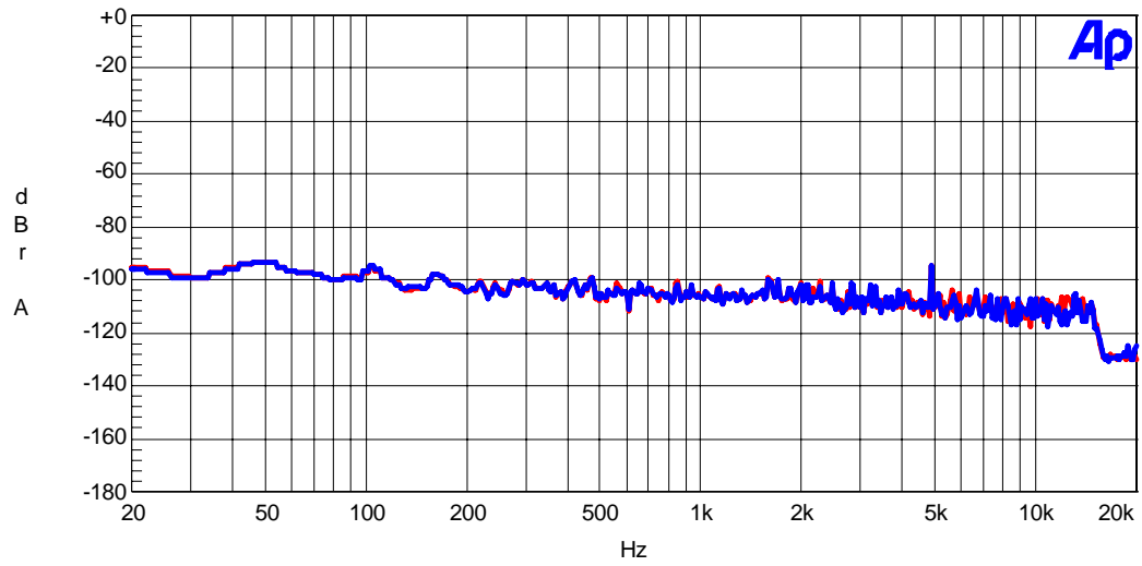
Figure. 15 Stereo mode FFT Plot (No Signal)
