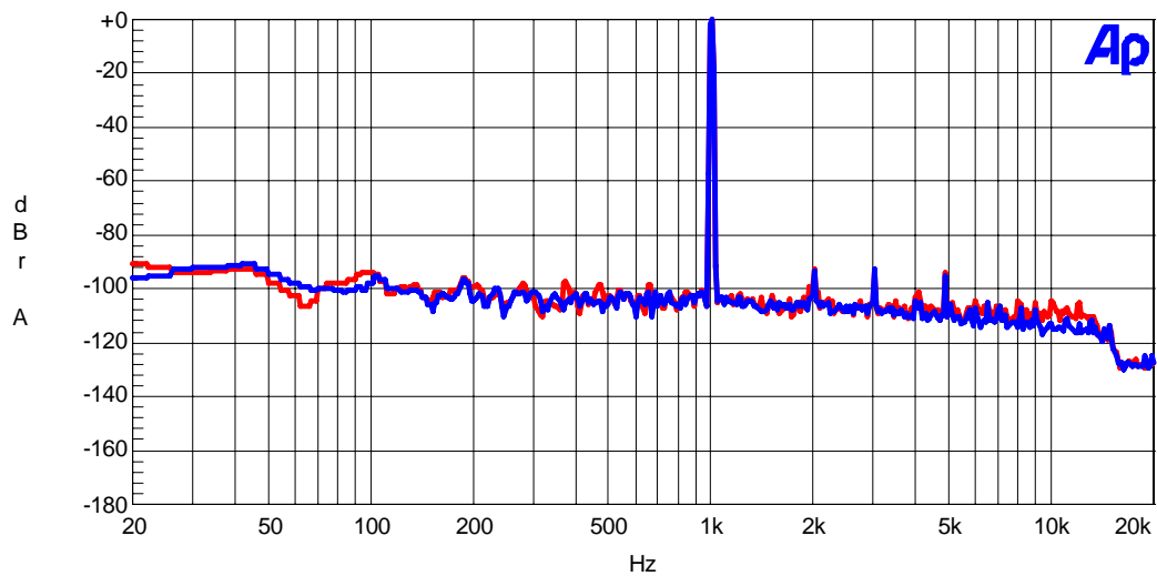
Figure. 14 Stereo mode FFT Plot (-1dB)
