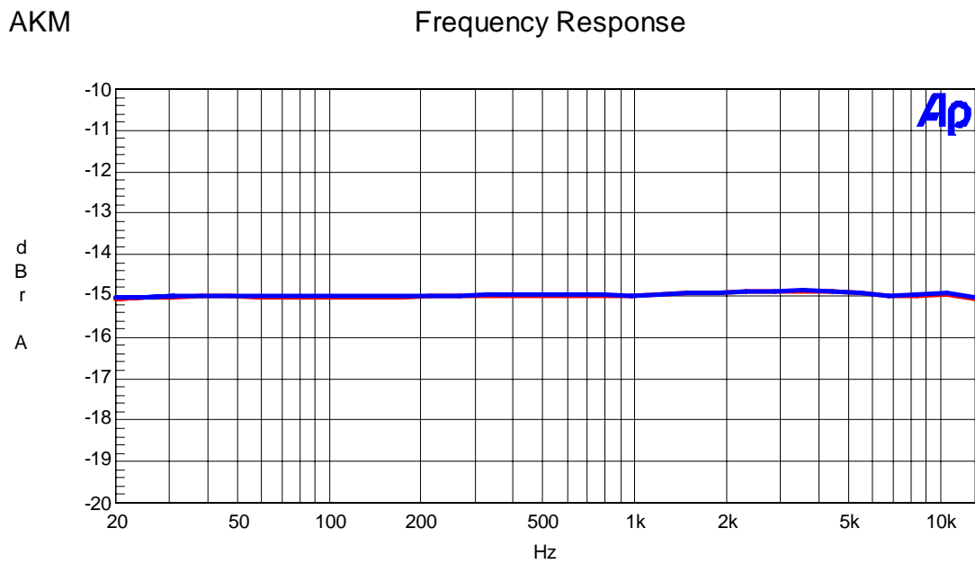
Figure. 12 Stereo mode Frequency Response (-15dB)
