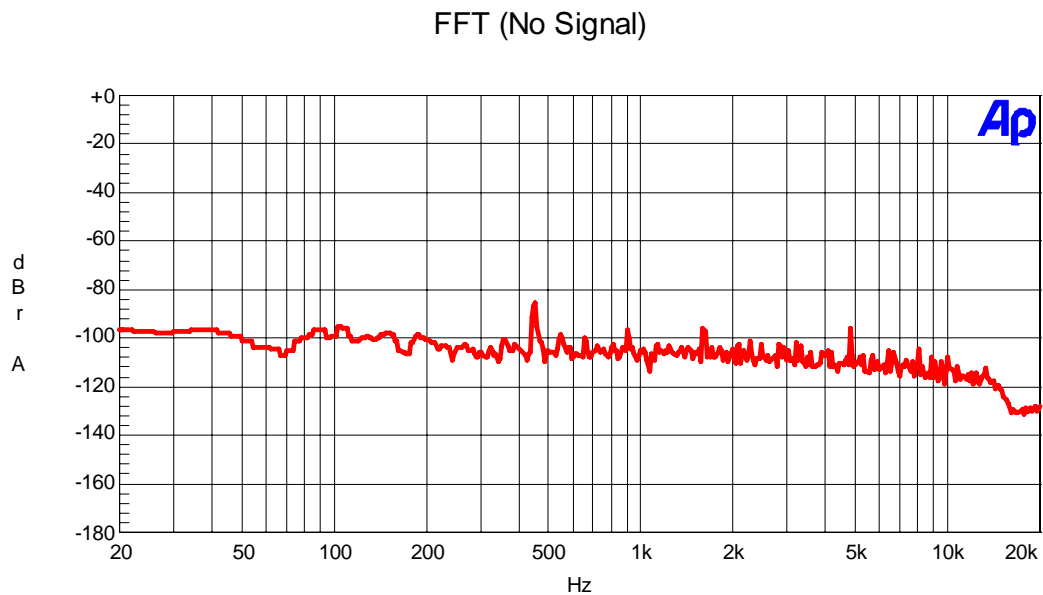
Figure. 21 Mono mode FFT Plot (No Signal)
