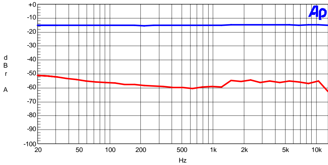
Figure. 13 Stereo Separation (Lch Off, Rch -15dB)
