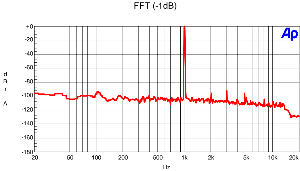
Figure. 20 Mono mode FFT Plot (-1dB)
