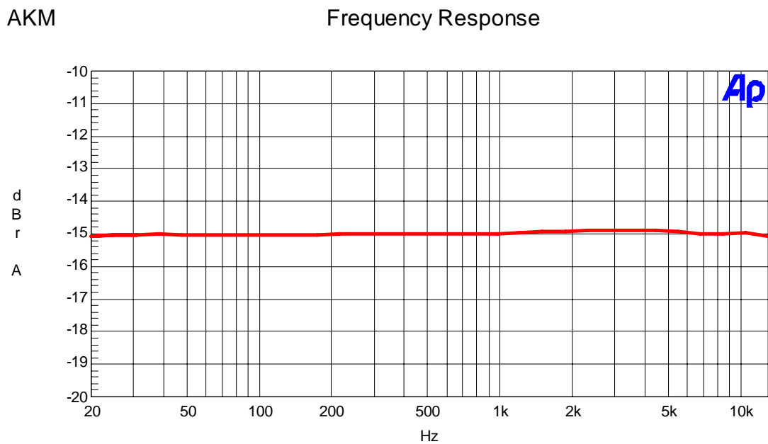
Figure. 19 Mono mode Frequency Response (-15dB)
