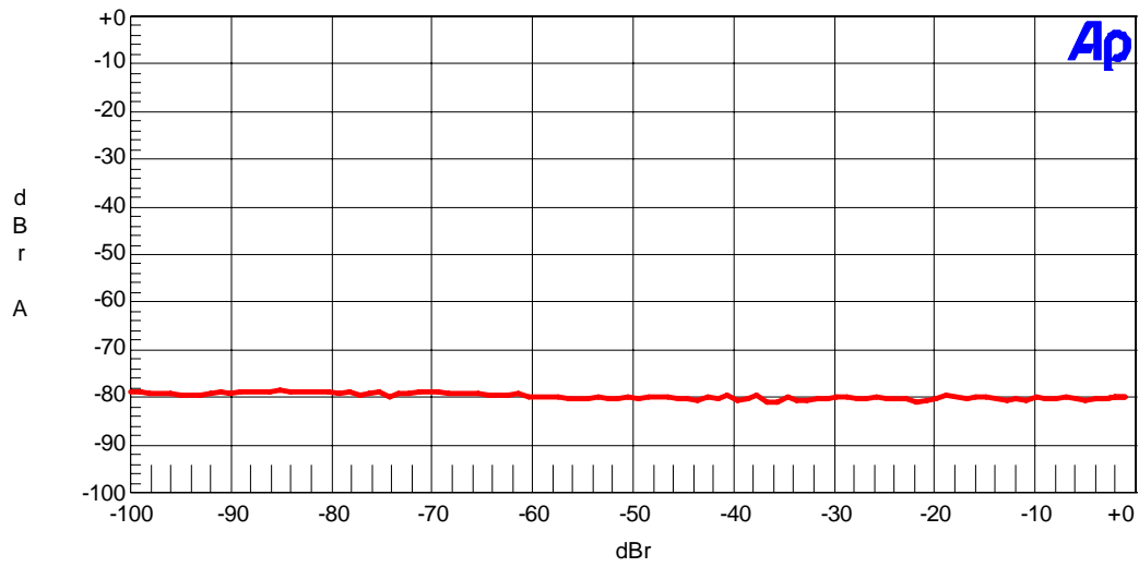
Figure. 16 Mono mode THD + N vs. Input Level (fin=1kHz)
