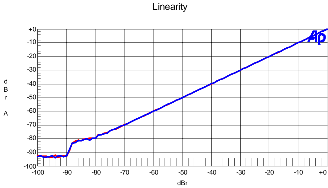
Figure. 11 Stereo mode Linearity (fin=1kHz)
