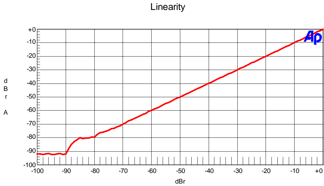
Figure. 18 Mono mode Linearity (fin=1kHz)
