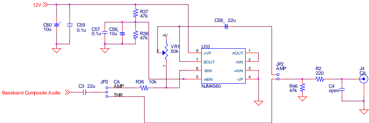
Figure. 3 Baseband Composite Audio signal output circuit
