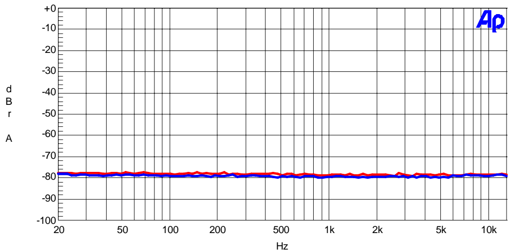
Figure. 10 Stereo mode THD + N vs. Input Frequency (-15dB)
