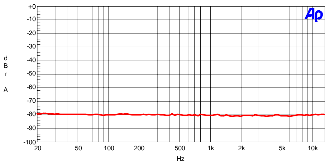
Figure. 17 Mono mode THD + N vs. Input Frequency (-15dB)
