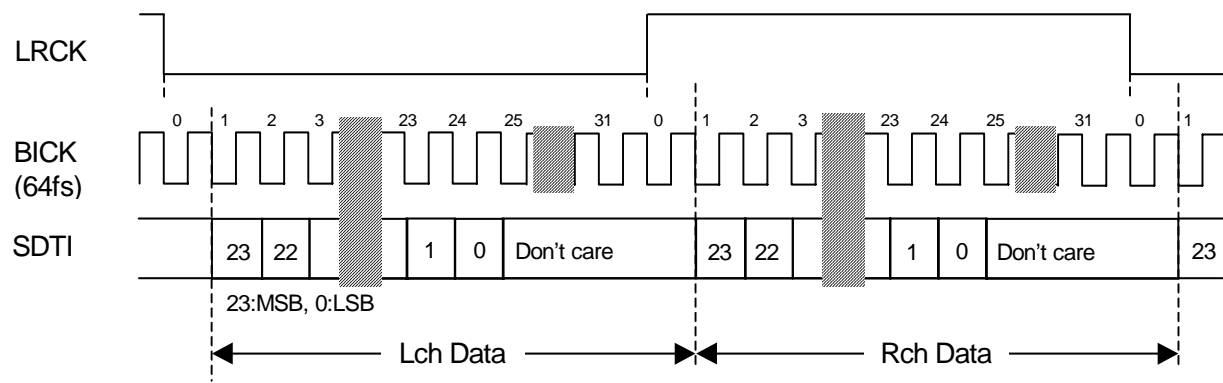
Figure 4. Mode 3 Timing
