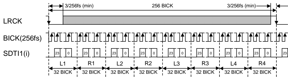
Figure 6. Mode 6 Timing
