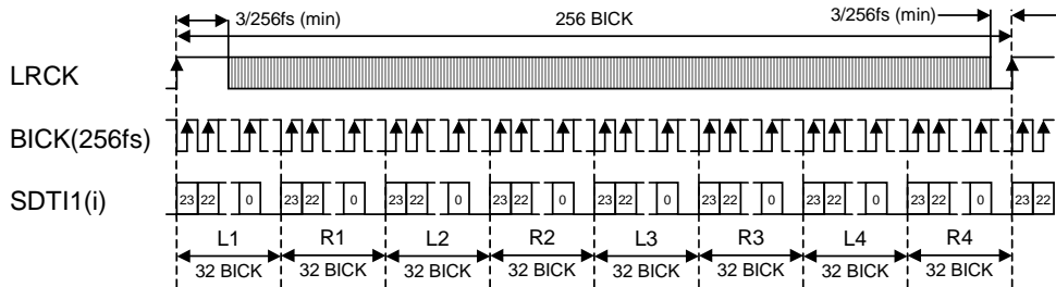
Figure 5. Mode 5 Timing
