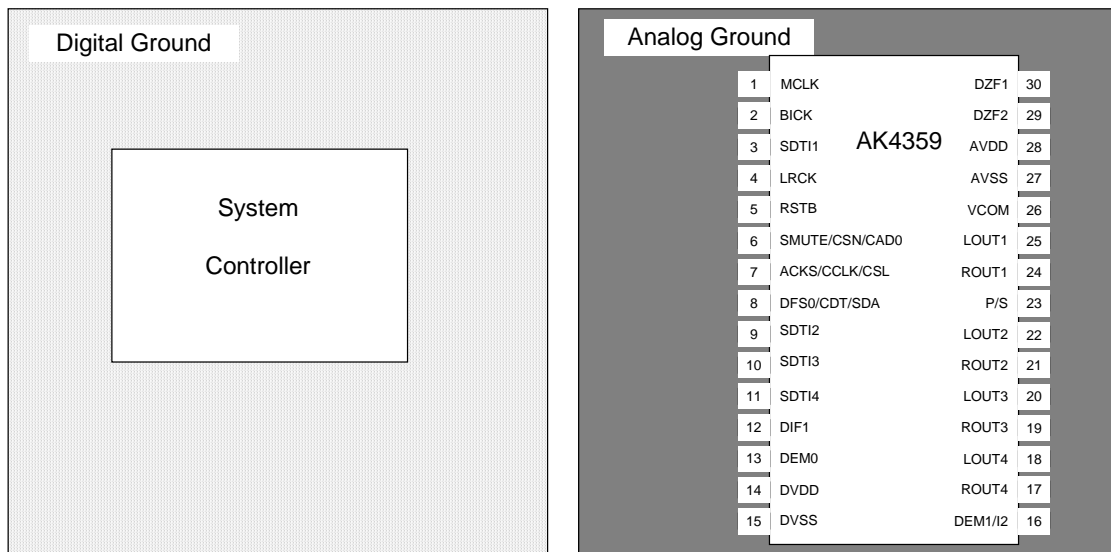
Figure 24. Ground Layout
