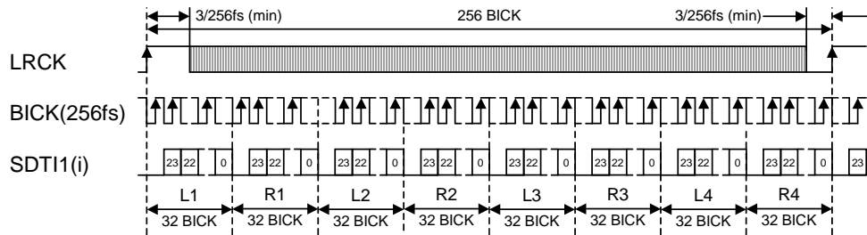
Figure 7. Mode 7 Timing
