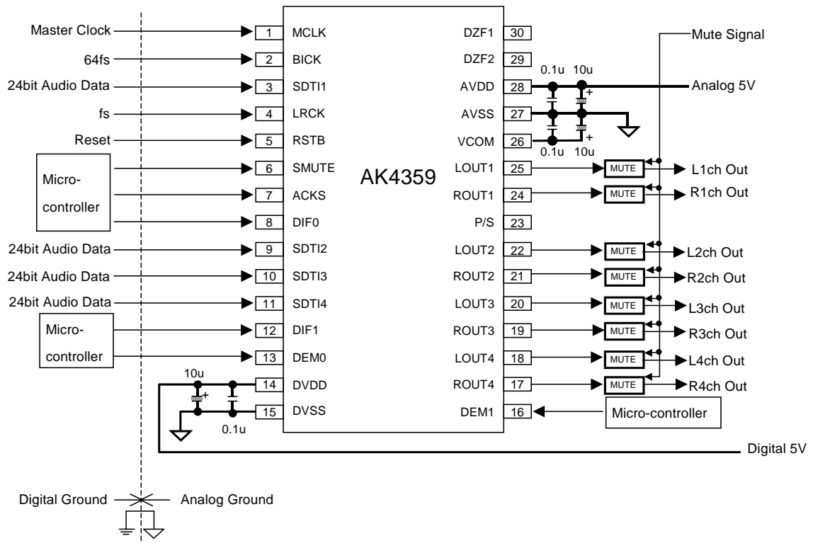
Figure 22. Typical Connection Diagram (Parallel Control Mode)
