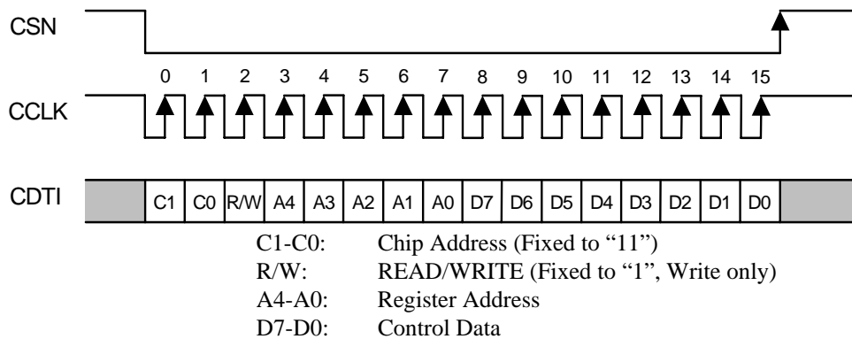
Figure 14. Control I/F Timing
