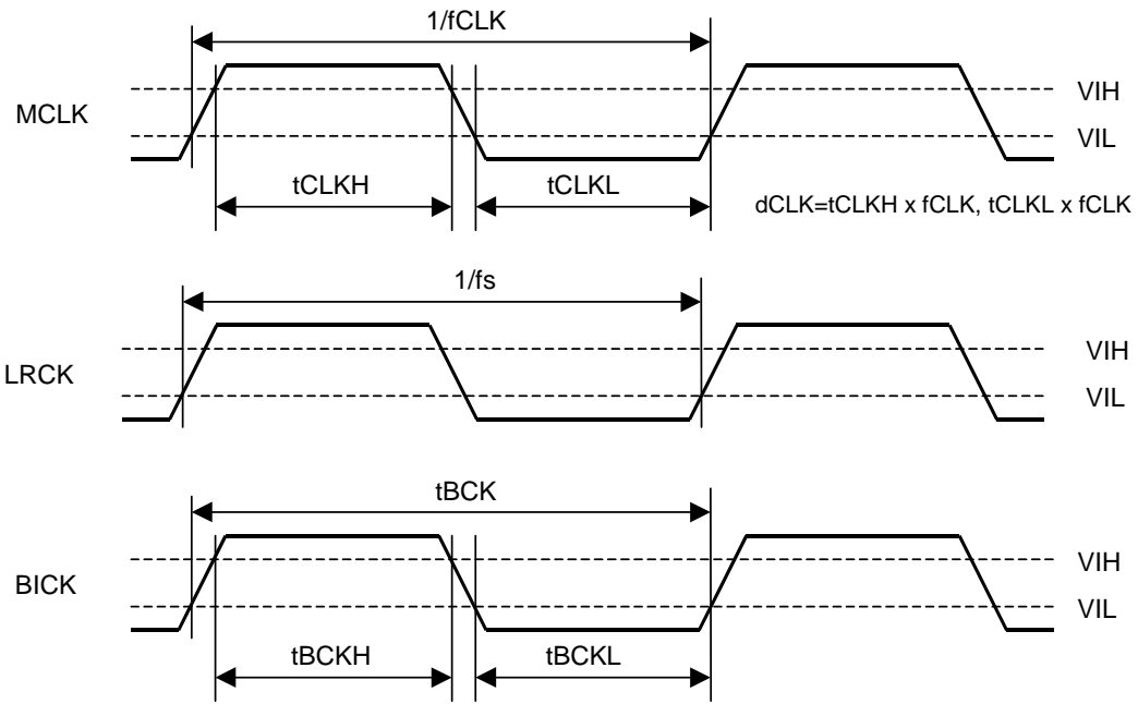
Clock Timing
