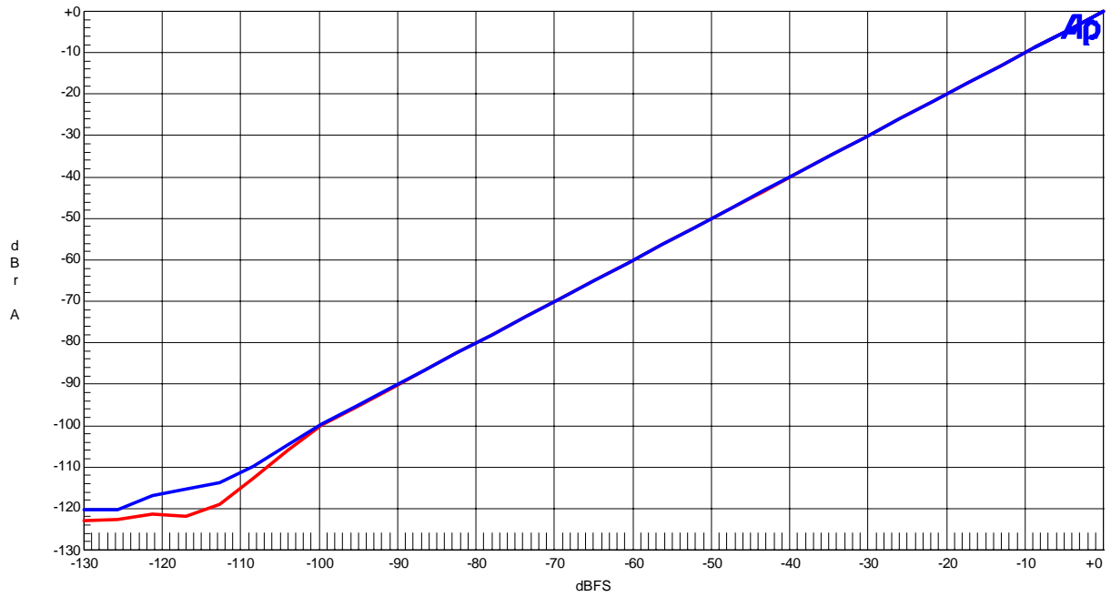
Figure 32. Linearity (fin=1kHz)
