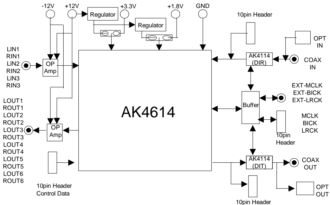
Figure1. AKD4614-A Block Diagram (*Circuit diagram and PCB layout are attached at the end of this manual.)
