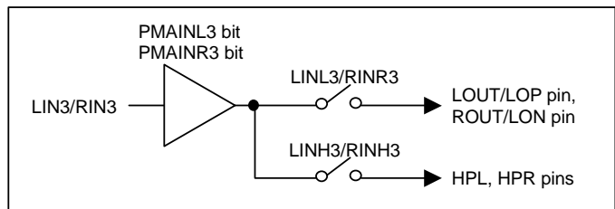
Figure 43. Analog Mixing Circuit (LIN3/RIN3: PLL is not available.)
