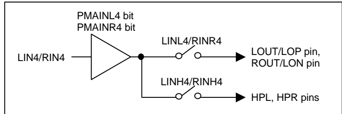
Figure 42. Analog Mixing Circuit (LIN4/RIN4)
