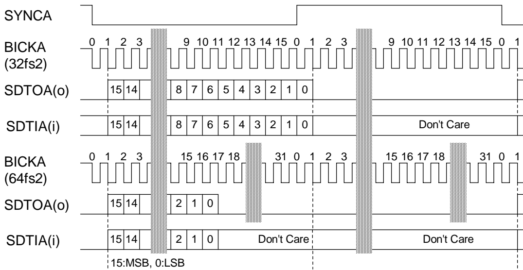
Figure 93. Timing of I 2 S
