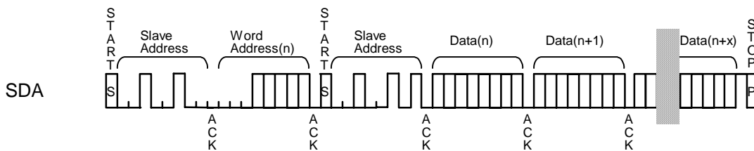
Figure 27. RANDOM READ
