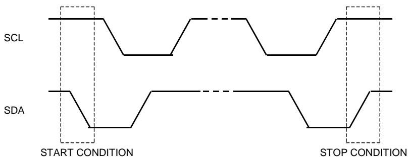
Figure 12. START and STOP Conditions
