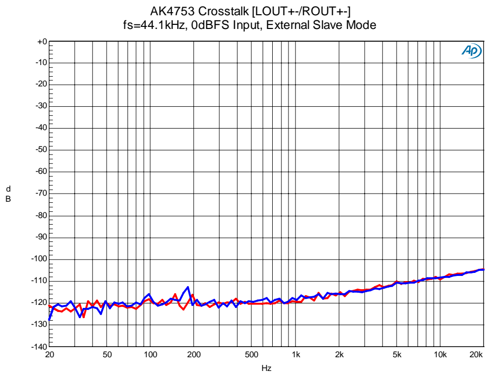
Figure 57. Crosstalk
