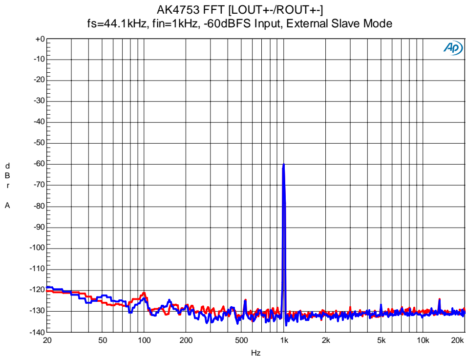
Figure 51. FFT(-60dB Input)
