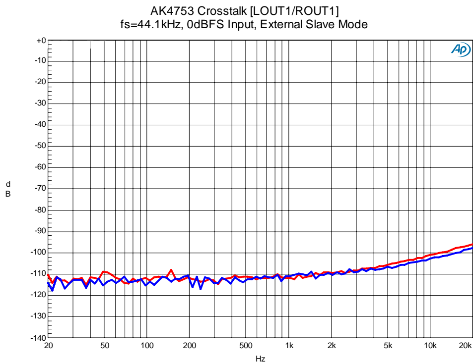
Figure 49. Crosstalk
