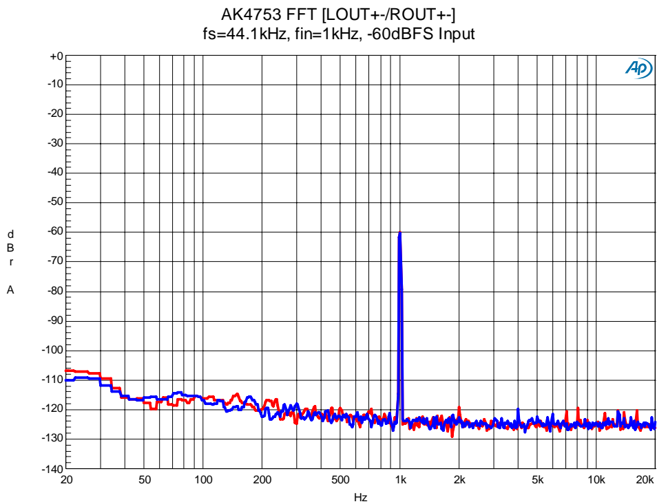
Figure 67. FFT(-60dBFS Input)
