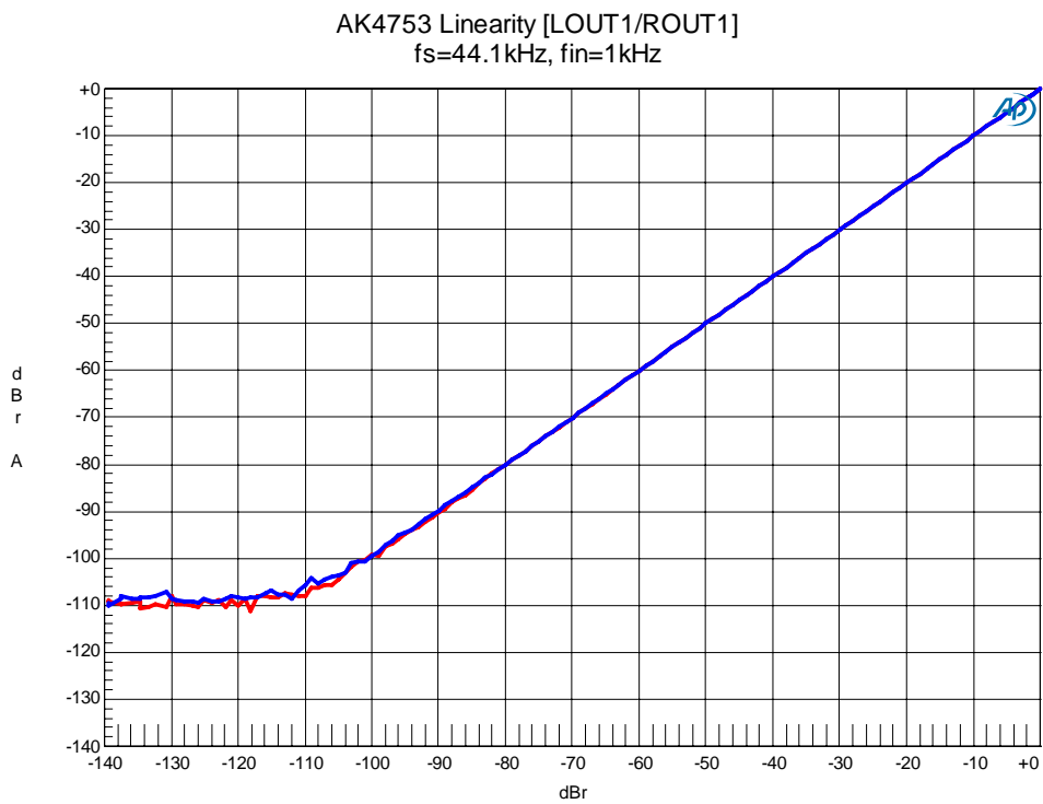
Figure 63. Linearity
