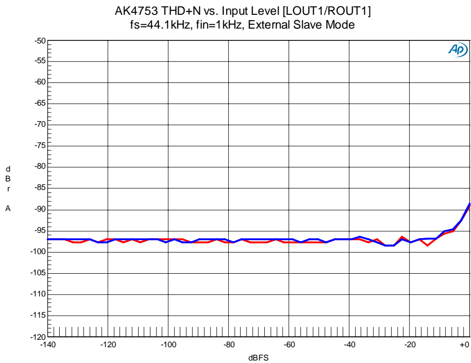
Figure 45. THD+N vs. Input Level
