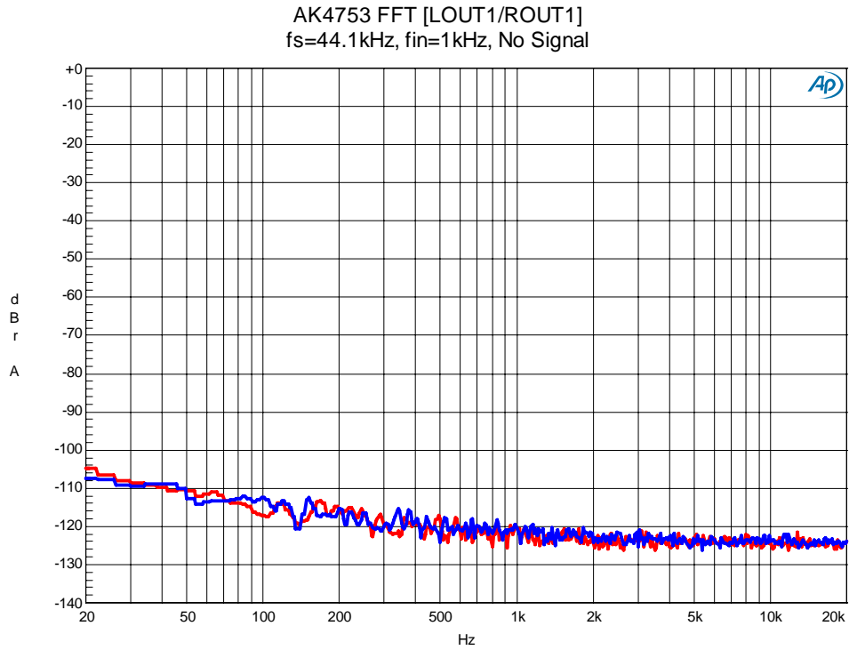
Figure 60. FFT(No Signal)
