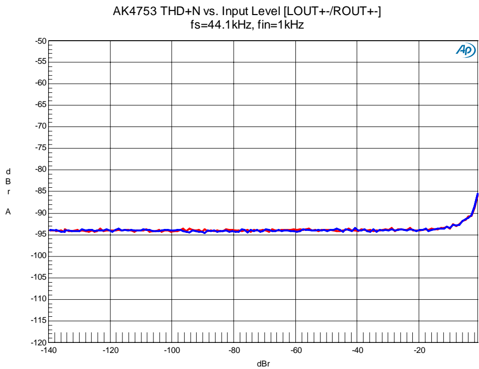
Figure 69. THD+N vs. Input Level
