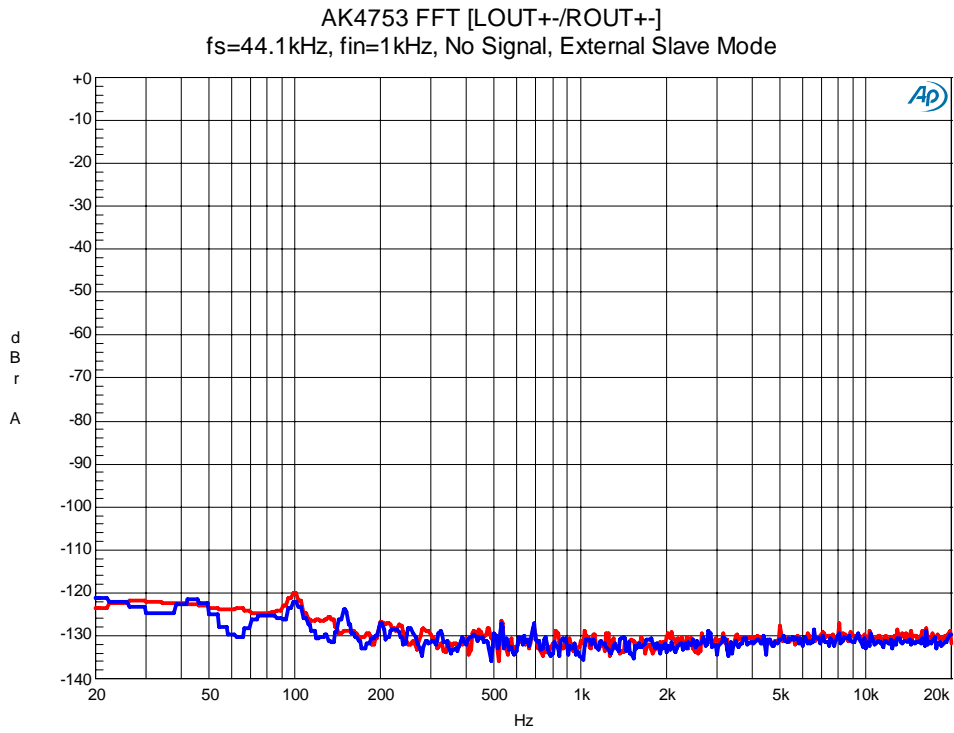
Figure 52. FFT(No Signal)
