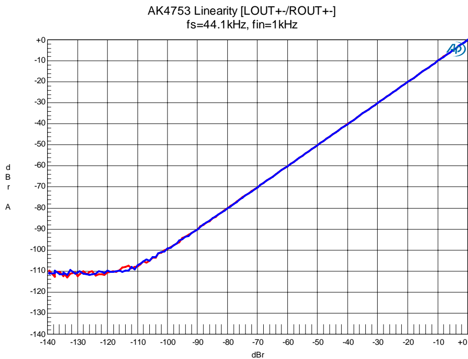
Figure 71. Linearity
