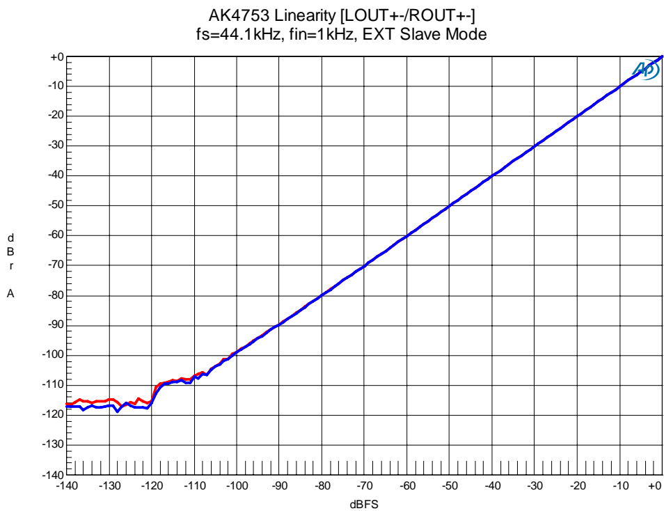
Figure 55. Linearity
