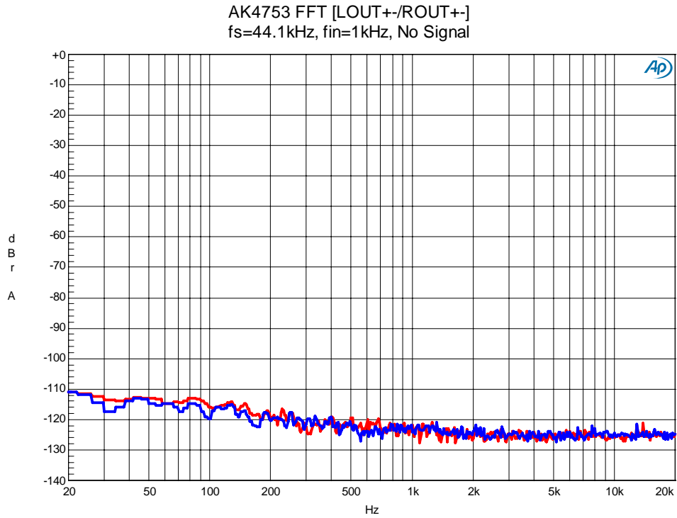
Figure 68. FFT(No Signal)
