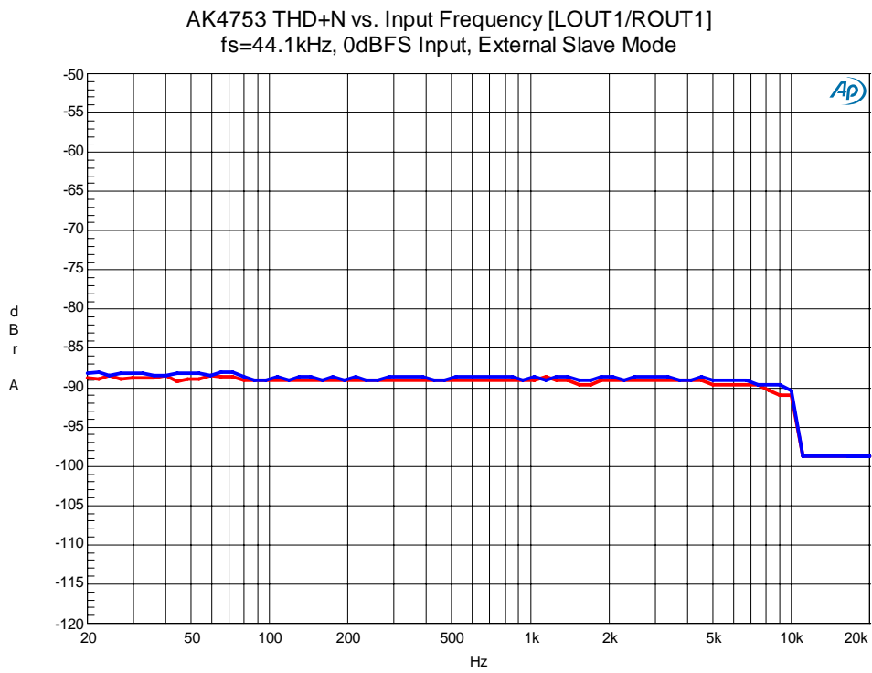
Figure 46. THD+N vs. Input Frequency
