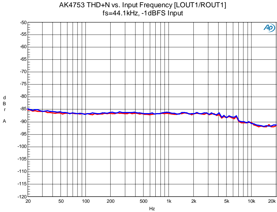
Figure 62. THD+N vs. Input Frequency
