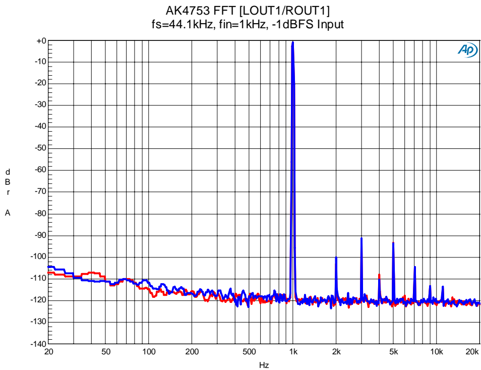
Figure 58. FFT(-1dBFS Input)
