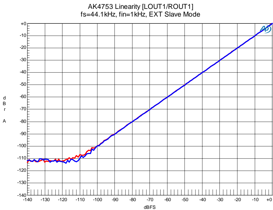
Figure 47. Linearity
