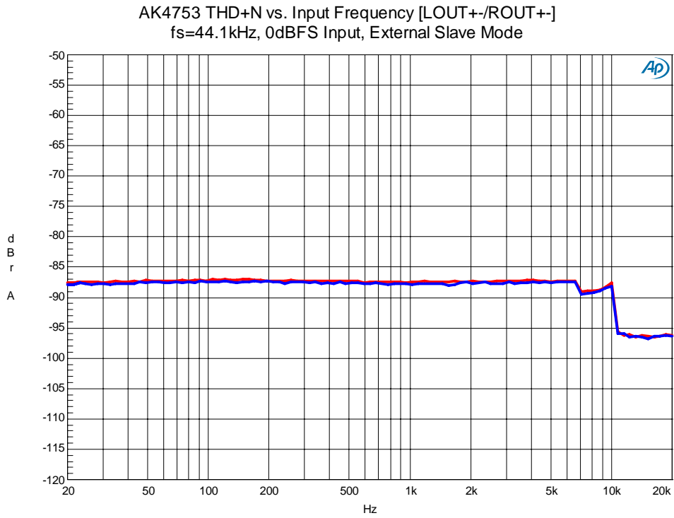
Figure 54. THD+N vs. Input Frequency
