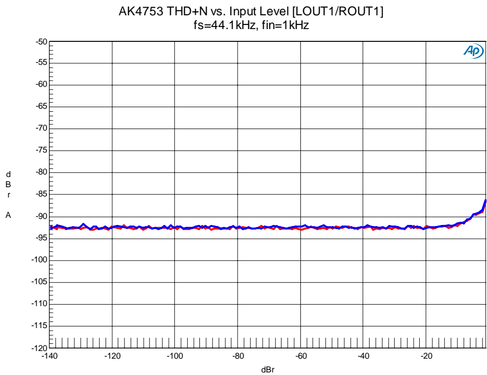
Figure 61. THD+N vs. Input Level
