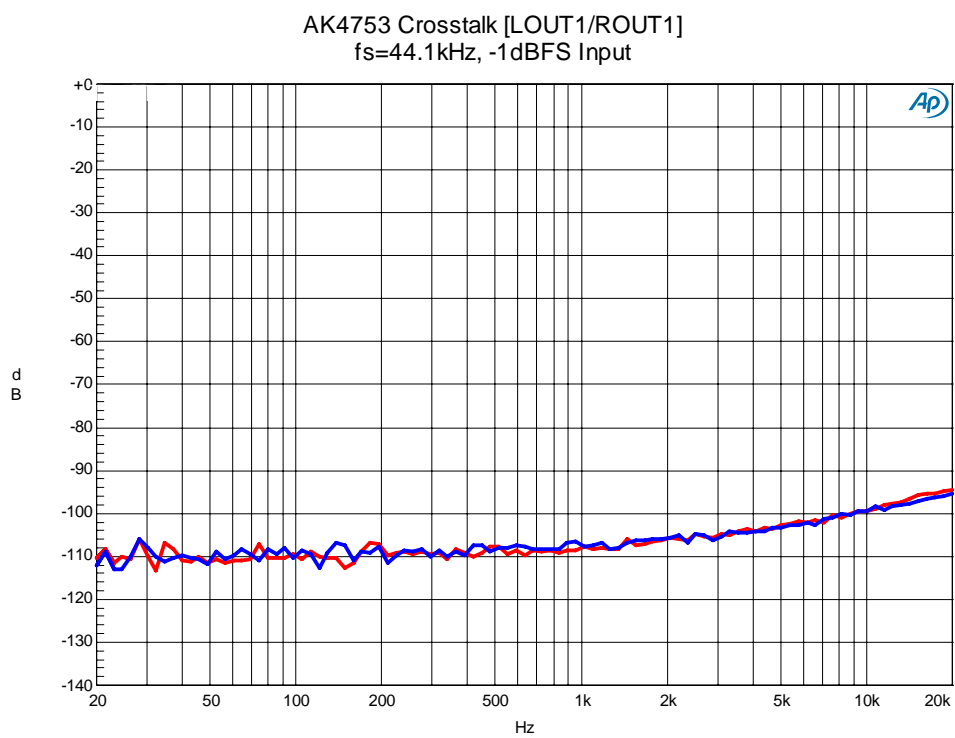
Figure 65. Crosstalk
