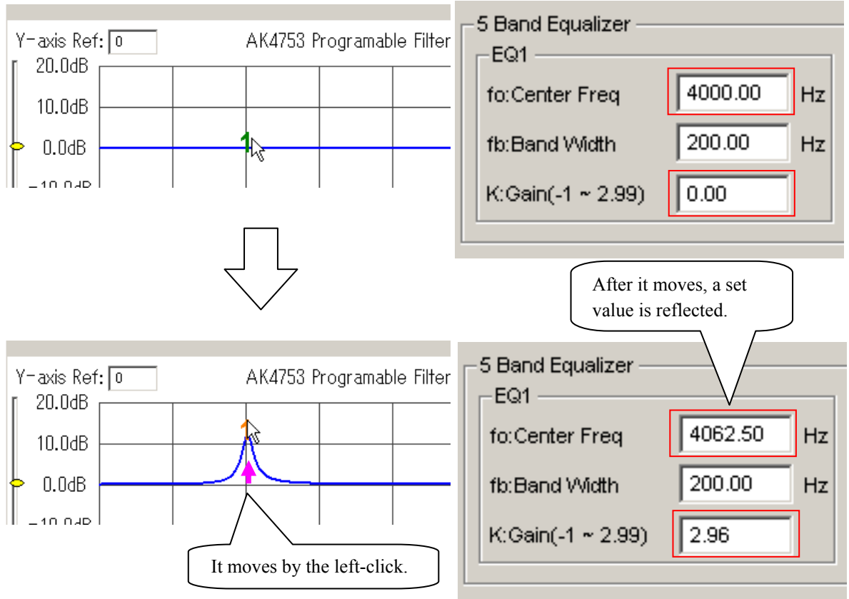
Figure 27. Filter Setting(Left-clicking operation)
