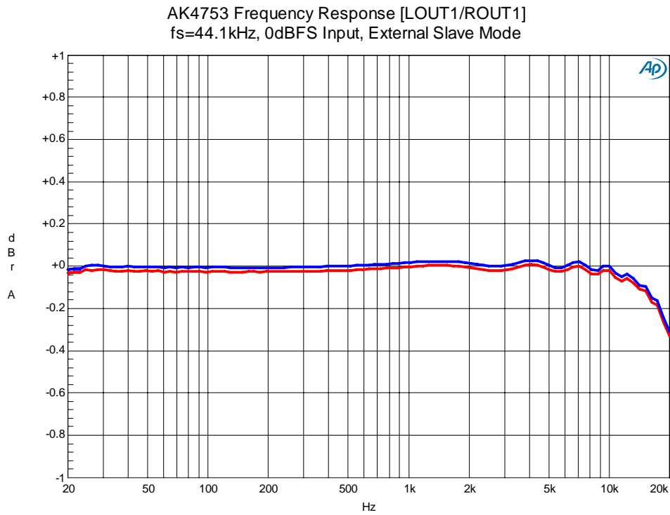
Figure 48. Frequency Response
