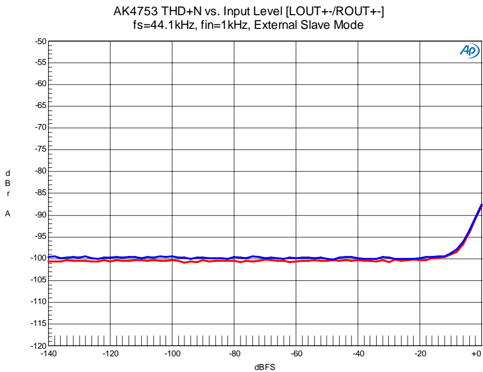
Figure 53. THD+N vs. Input Level
