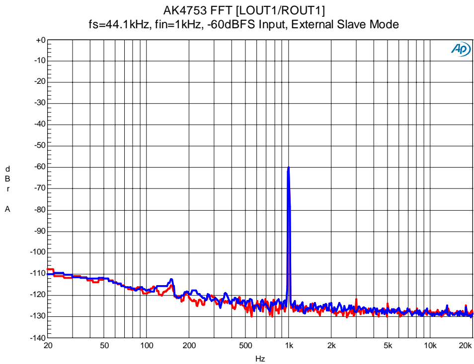
Figure 43. FFT(-60dB Input)
