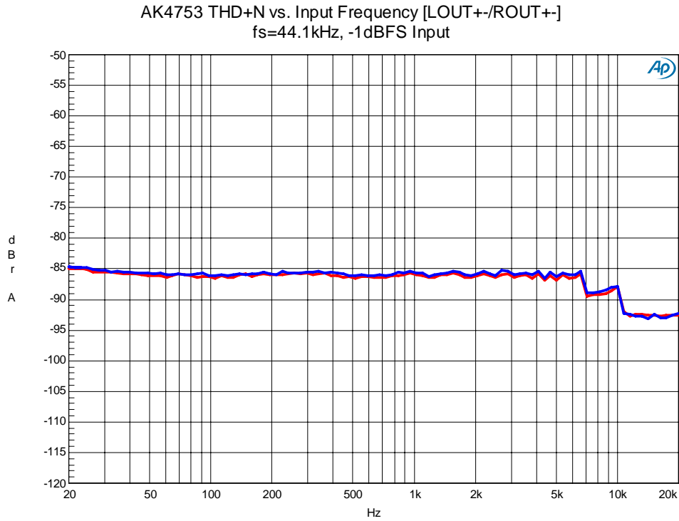
Figure 70. THD+N vs. Input Frequency
