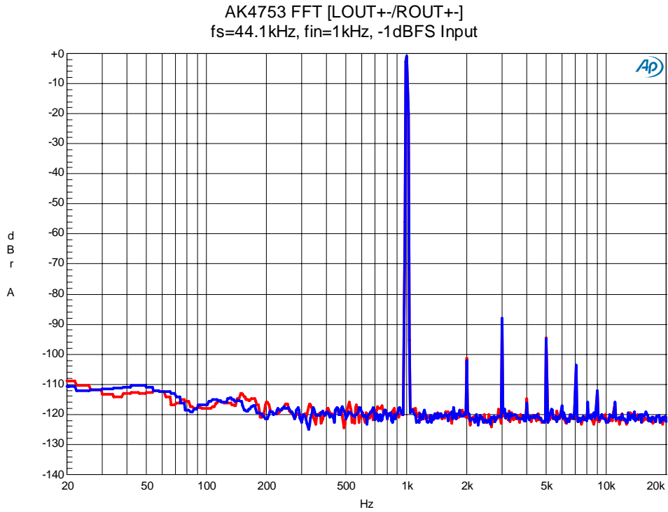
Figure 66. FFT(-1dBFS Input)
