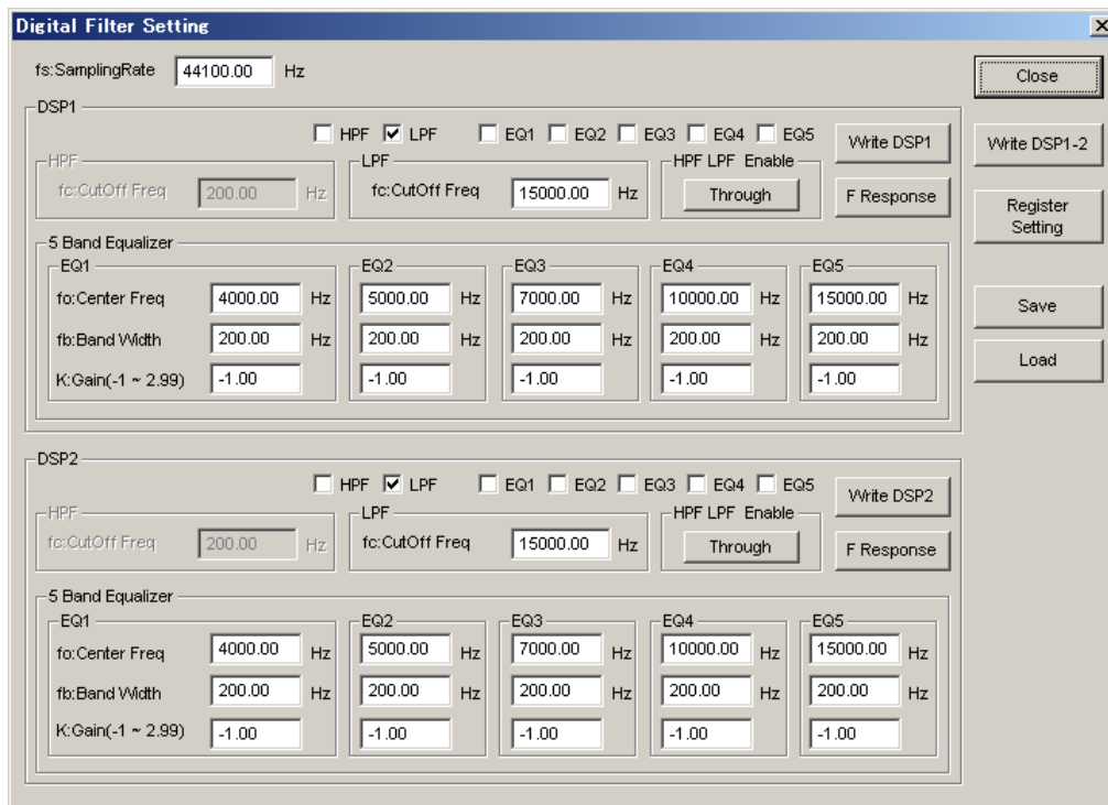
Figure 23. Window of [Digital Filter Setting]
