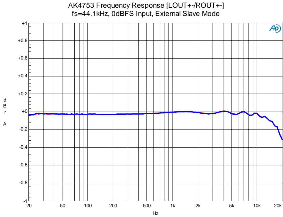
Figure 56. Frequency Response
