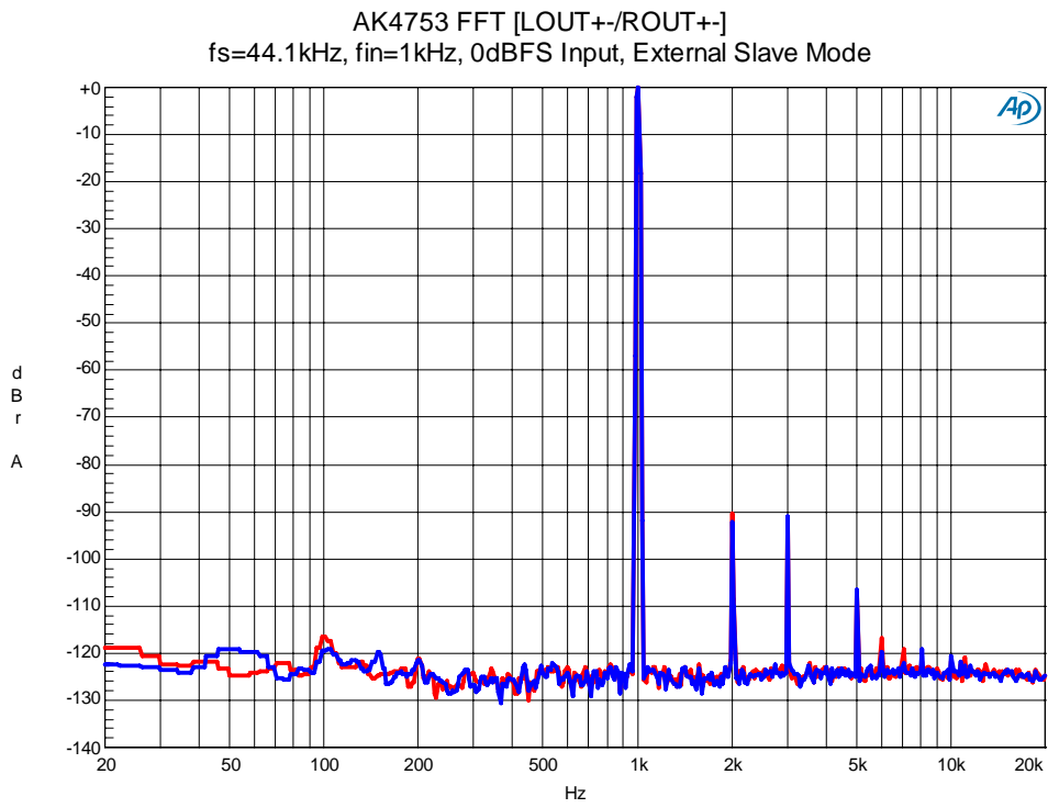
Figure 50. FFT(0dBFS Input)
