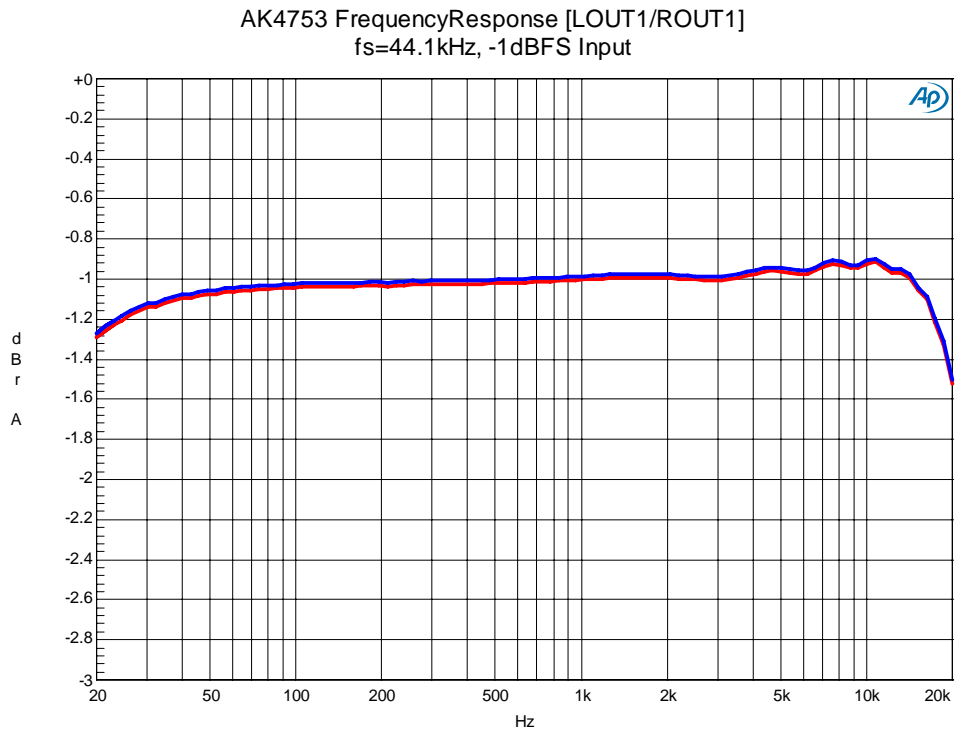
Figure 64. Frequency Response
