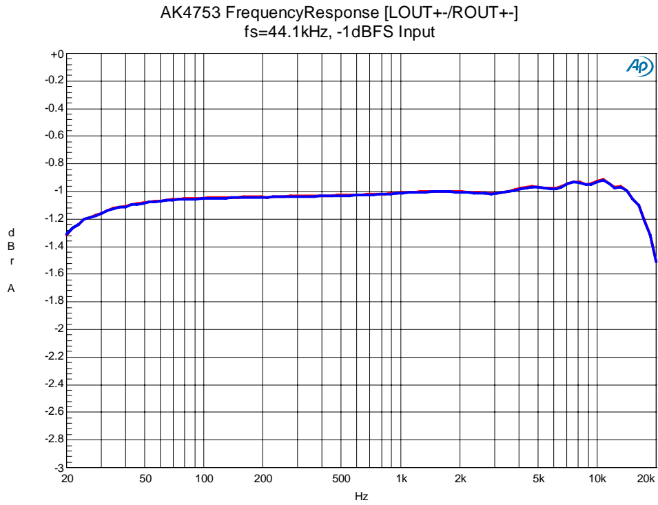
Figure 72. Frequency Response
