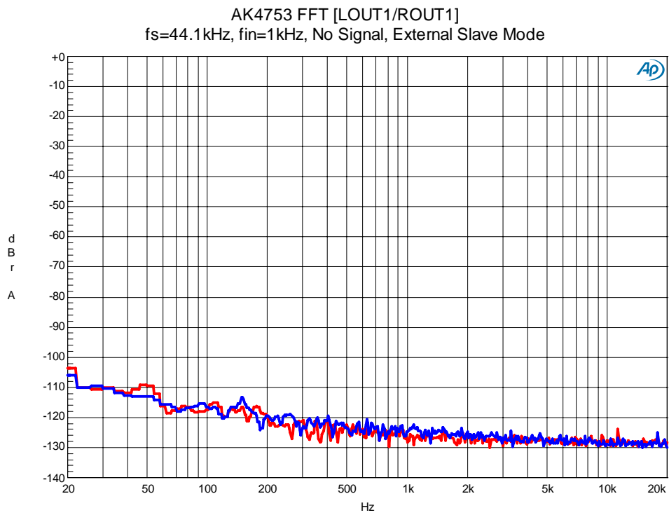
Figure 44. FFT(No Signal)
