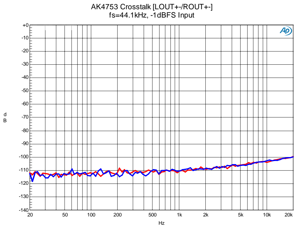
Figure 73. Crosstalk
