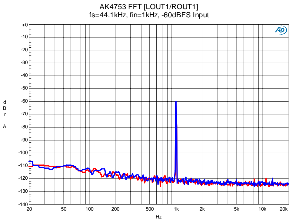
Figure 59. FFT(-60dBFS Input)
