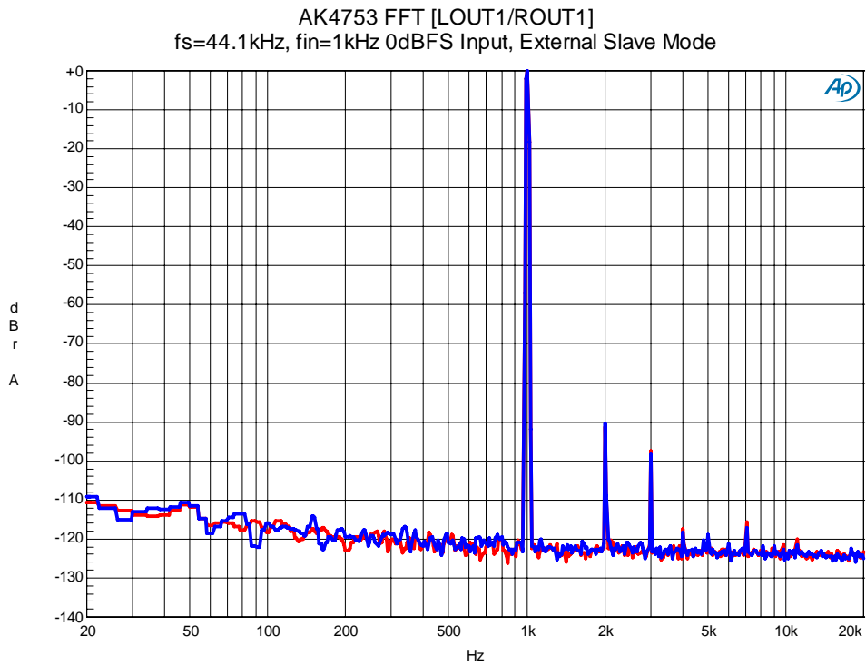
Figure 42. FFT(0dBFS Input)
