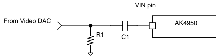
Figure 2. External Resistor of Video Signal Input pin
